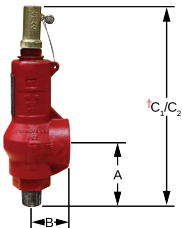
1" THREADED VALVE
