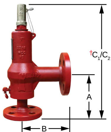
1" FLANGED VALVE
