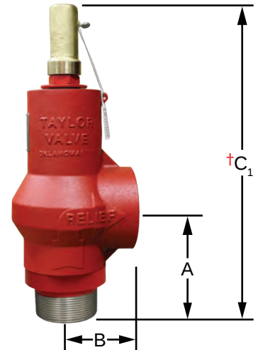
3" THREADED VALVE
