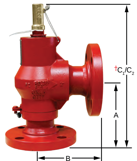
2" FLANGED VALVE
